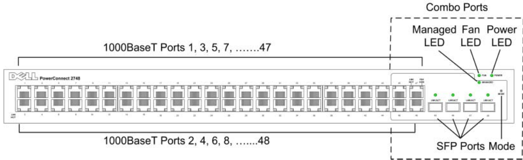
Figura 2-7. Panel frontal de PowerConnect 2748
