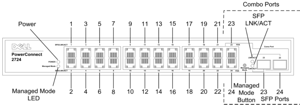
Figura 2-5. Panel frontal de PowerConnect 2724
