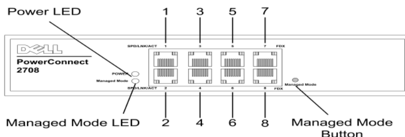
Figura 2-1. Panel frontal de PowerConnect 2708
